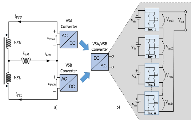
High-Voltage DC/AC Converters power supply for VSS coils
